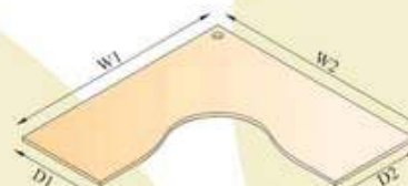
CURVILINEAR TOP (TYPE-2) W1=1500,1650,1800 W2=1500,1650,1800 D1=500,600,750 D2=500,600,750
