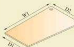
CALL CENTER TOP (TYPE-2) W1=1050,1200,1350,1500,1800 D1=450,500,600,750,900 D2=500,600,750,900,1050
