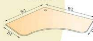
CURVILINEAR TOP (TYPE-3) W1=1200,1350,1500,1650,1800 W2=1200,1350,1500,1650,1800 D1=450,500,600,750 D2=450,500,600,750
